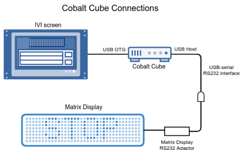
Figure 2: Connectivity diagram for the Matrix Display
