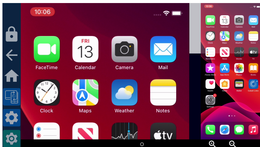
Figure 13: Zoom mode
